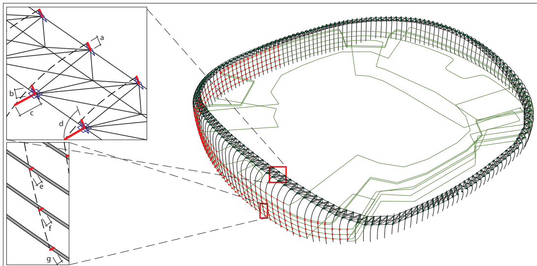
Figure 5.11: Measuring tolerances.
