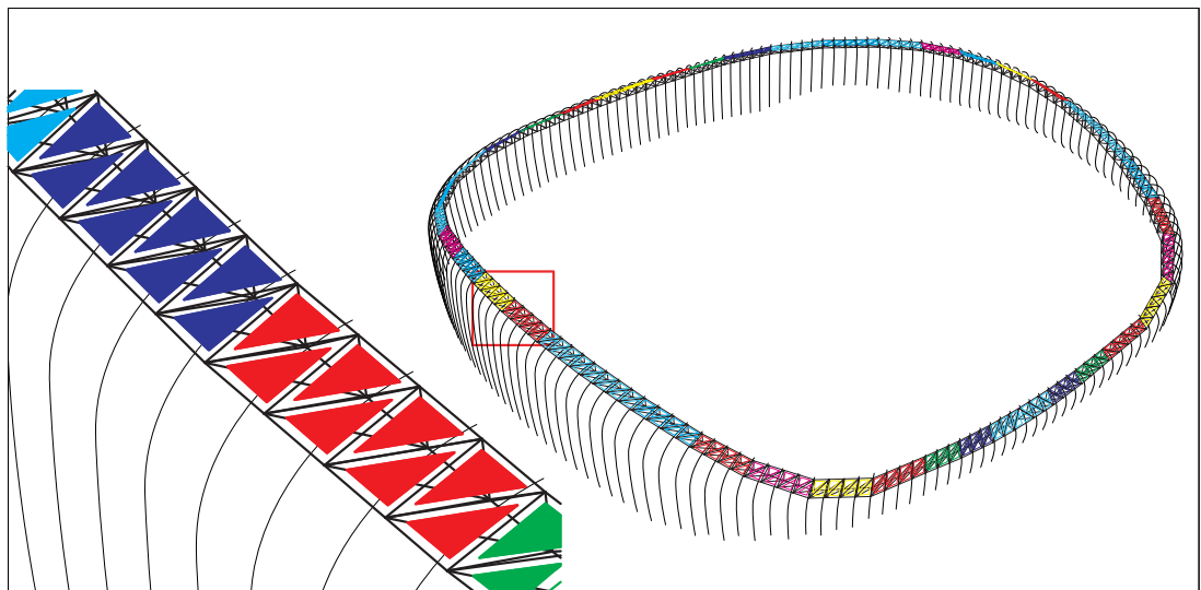
Figure 5.13: Acoustic panels rationalised and grouped by colour.
