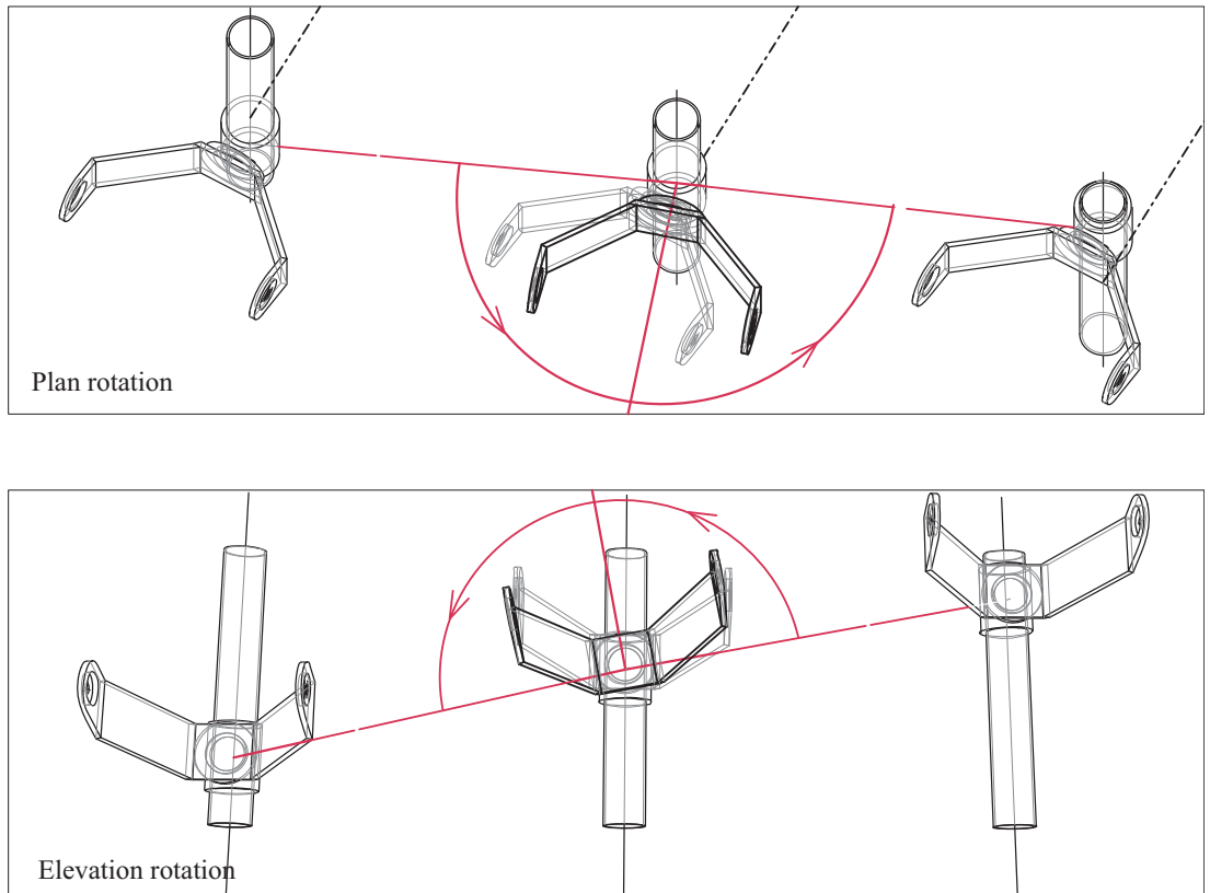
Figure 5.8: Bracket rotation principle.
