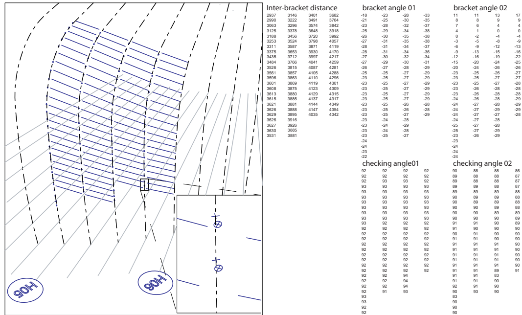
Figure 5.10: Information issued for one facade bay.
