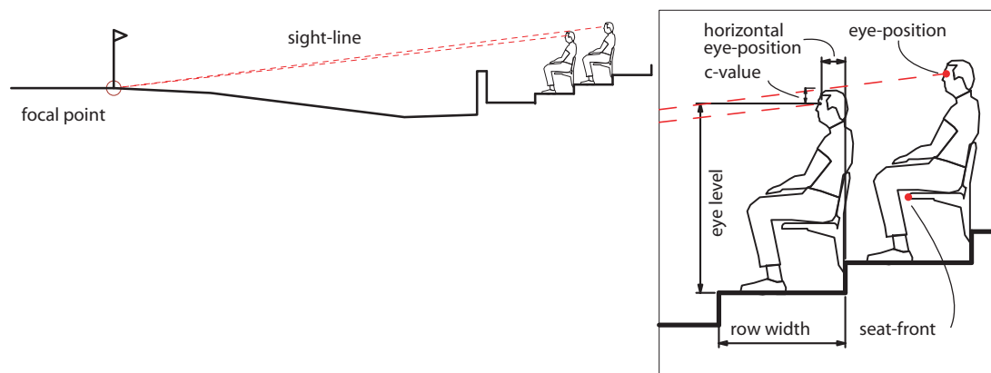
Figure 6.1: C-value method.
